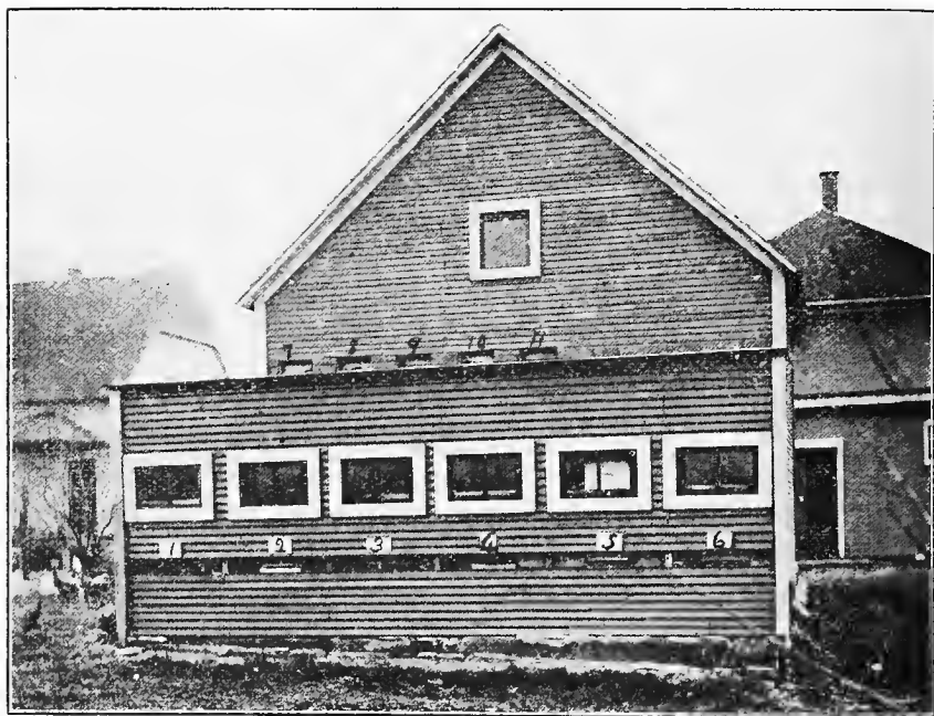
Exterior of a combined Poultry and Bee house at the author's home, showing where bees are kept in barn loft and poultry house,
